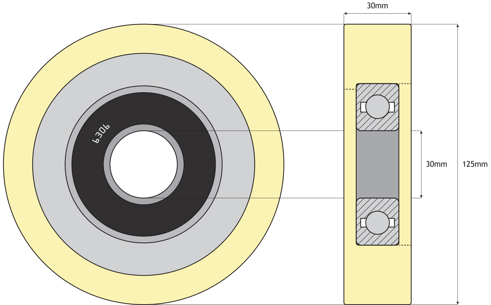
*6306RS Bearing
