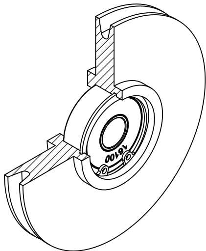
*16100 Bearing
