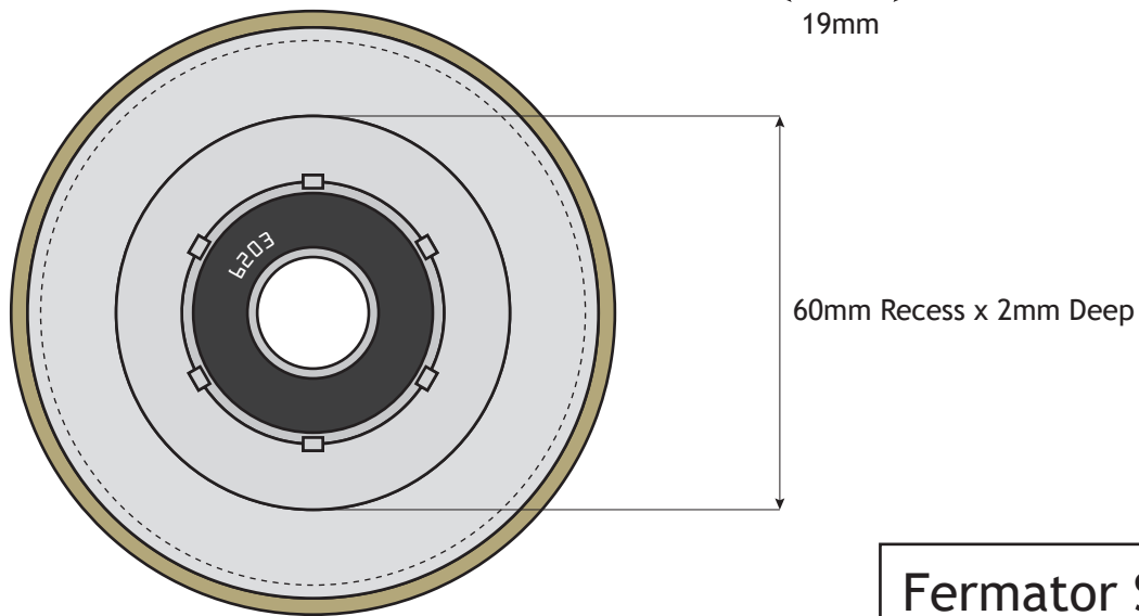
*6203 Bearing
